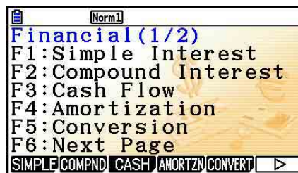
Financial 1 screen
