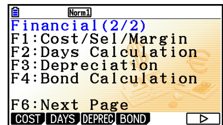
Financial 2 screen
